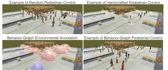
Fig. 1. Different methods for specifying pedestrian behaviors in SEAN 2.0. The Behavior Graph method is a novel approach that uses an environmental graph-based annotation (bottom-left) to generate behavior (bottom-right).
