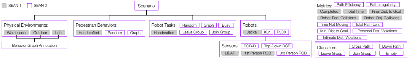
Fig. 3. SEAN 2.0 system architecture including components that were re-used or adapted from SEAN 1.0 (rounded box, grey) and new to SEAN 2.0 (purple). Connections denote relationships between components in a Scenario. The Scenario, Metrics, and Classifiers are part of the SEAN 2.0 Unity API and exist for all scenes. The SEAN 1.0 Trial Runner [12] is superseded by Robot Tasks and the Metrics system in SEAN 2.0. Warthog is the only robot in SEAN 1.0 which is not in SEAN 2.0 due to its unwieldy size relative to people. See the text for details.
