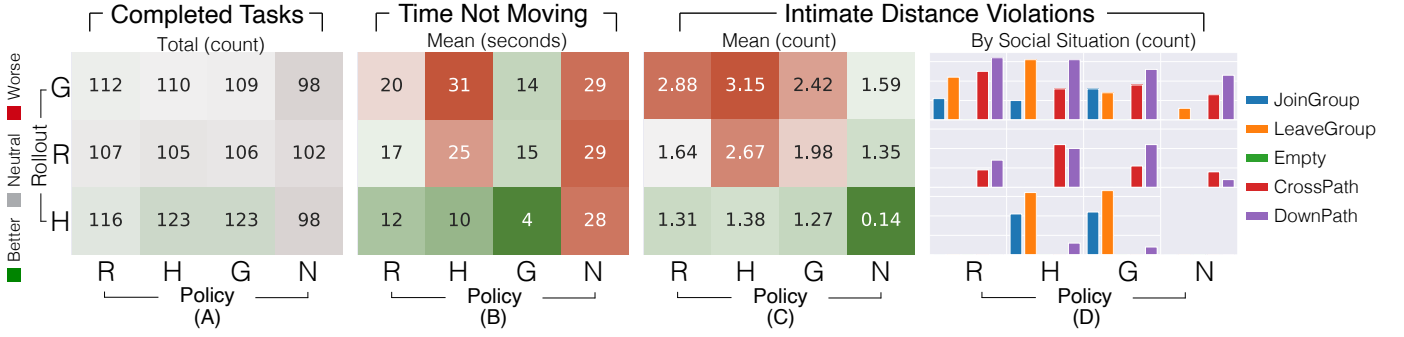
Fig. 4. Select results for 4 policies in 3 scenarios aggregated over 123 episodes. The three learned policies are trained on data from the Behavior Graph (G), Random (R), and Handcrafted (H) methods of pedestrian control. We also evaluate the ROS Navigation (N) policy with social cost layers [49]. Three metrics are shown: Completed Tasks (A), Time Not Moving (B), and Intimate Distance Violations (C and D). Values for Time Not Moving are computed in seconds and averaged over all episodes. All other plots show the total or average count of the occurrences of the metric over all episodes. The percentage gain for a specific metric can be calculated between grid-cells. For example, the Behavior Graph policy spends 55% less Time Not Moving than the Handcrafted policy when rolled out in the Behavior Graph environment.
